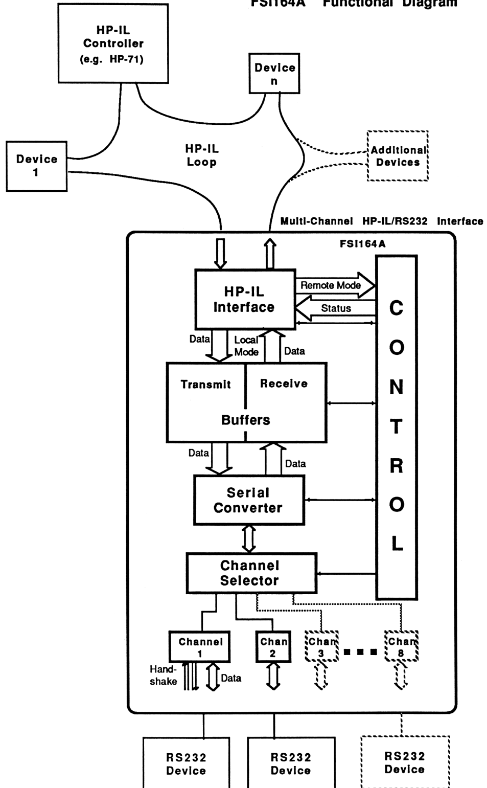
FSI164A Functional Diagram
