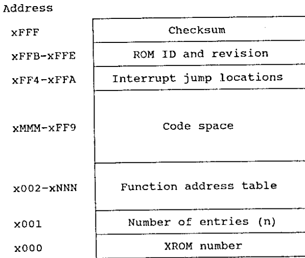
Fig. 15, ROM block structure
