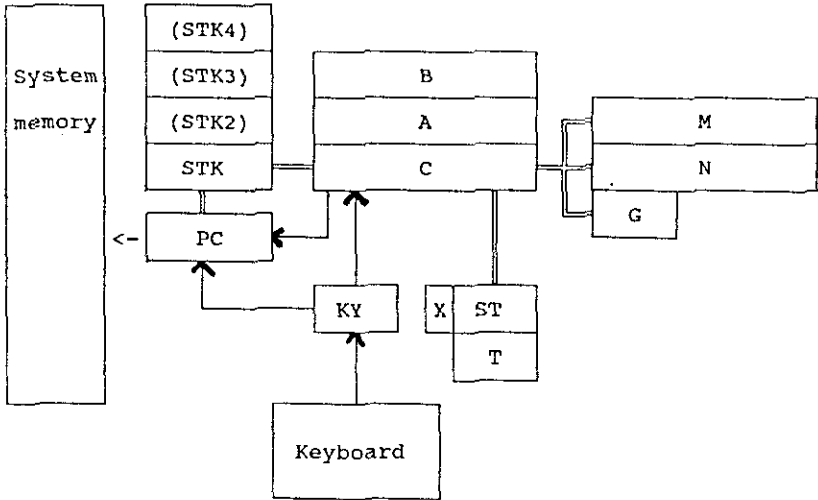
Fig. 16, CPU register connections
