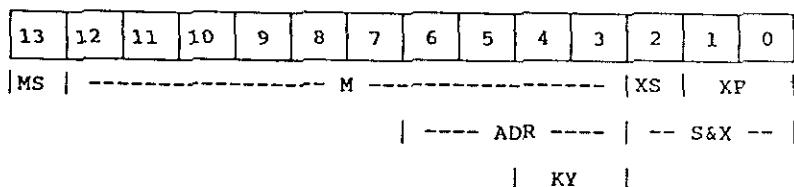
Fig. 17, Structure of registers
