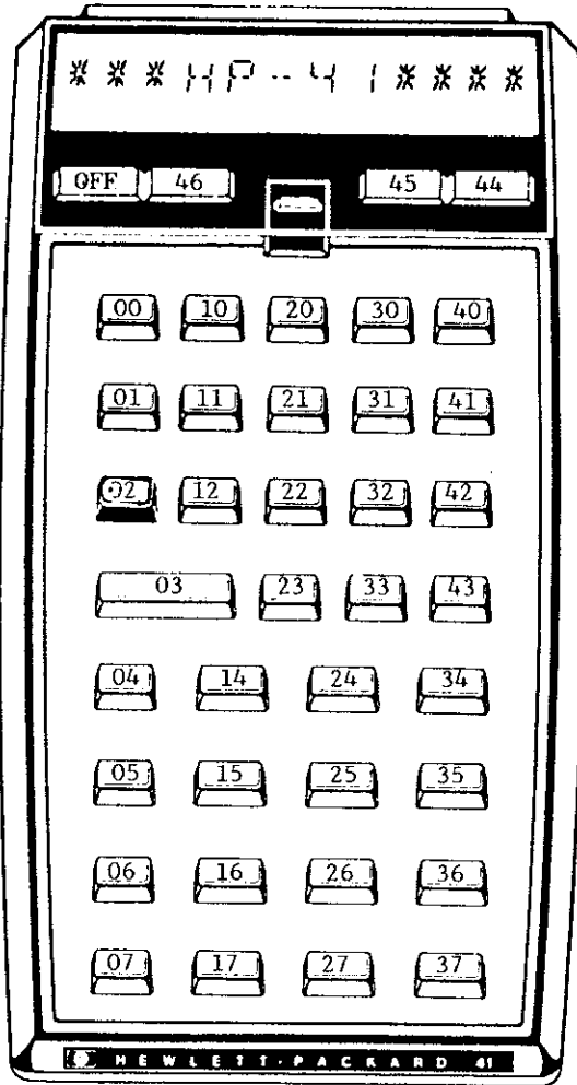
Fig. 23, Keycodes returned by 0E50 subroutine
