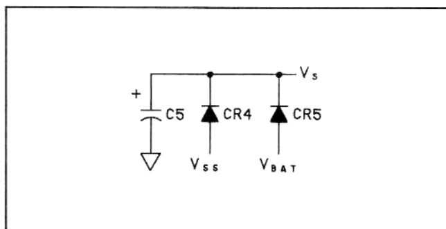
Figure 2-10. CMOS Power Supply Circuitry
