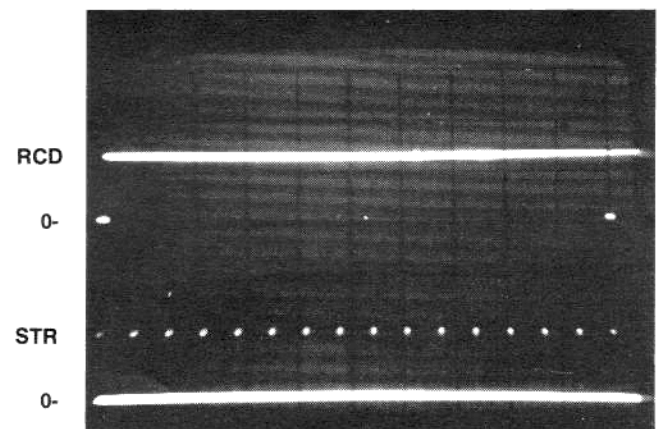
TEST POINTS: RCD: PIN 21 OF ACT (LU4) STR: PIN 11 OF ROM 0 (LU1) OSCILLOSCOPE TIME BASE: 5 MS/DIV VERTICAL GAIN: 2 V/DIV
