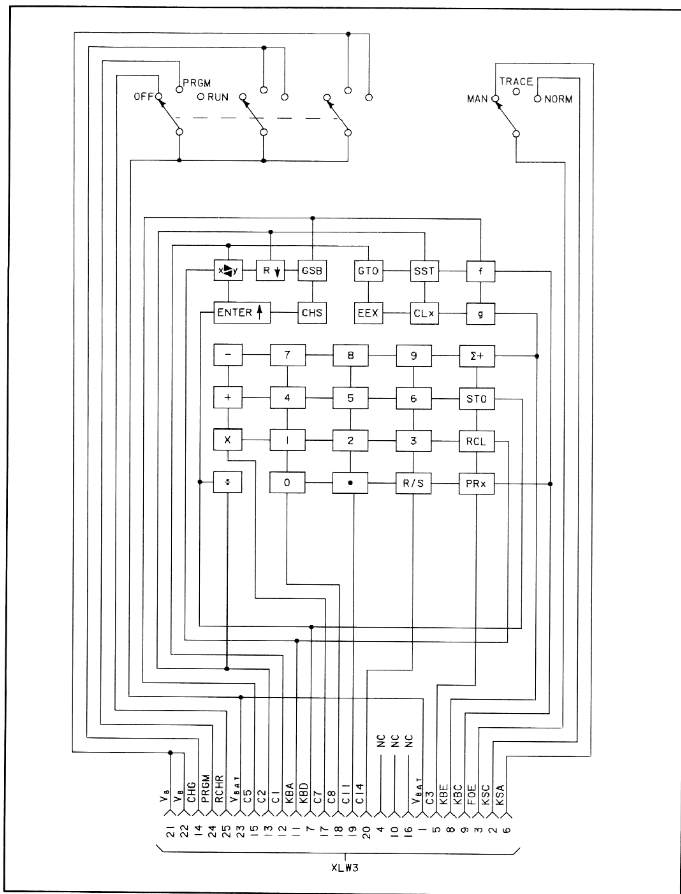
Figure 4-12. Keyboard PCA Schematic Diagram
