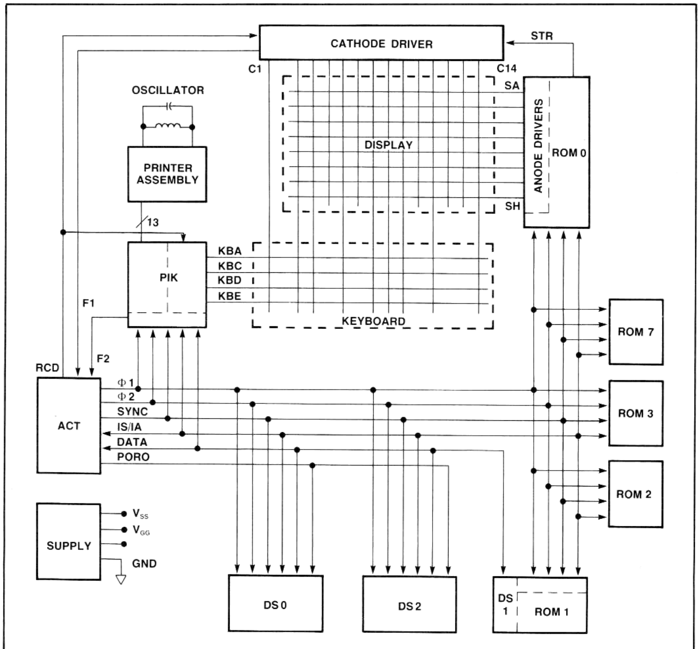
Figure 2-1. HP-19C Block Diagram
