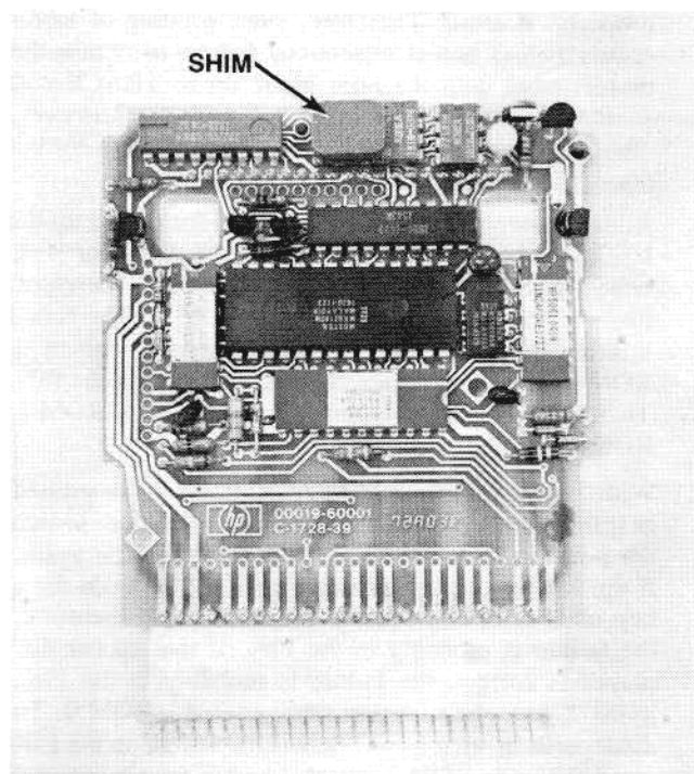
Figure 4-9. Rubber Shim Position
