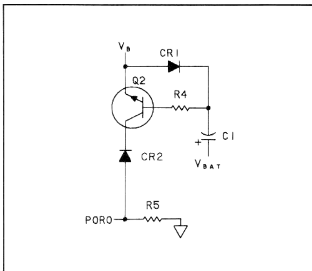
Figure 2-13. Power-Off Circuitry
