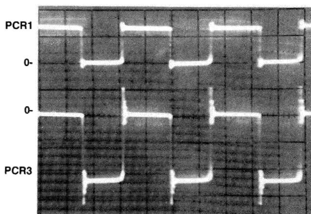
TEST POINTS: ANODES OF PCR1 AND PCR3 OSCILLOSCOPE TIME BASE: 2 \mu S/DIV VERTICAL GAIN: 5 V/DIV
