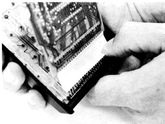
Figure 3-4. Securing Logic PCA to Keyboard PCA
