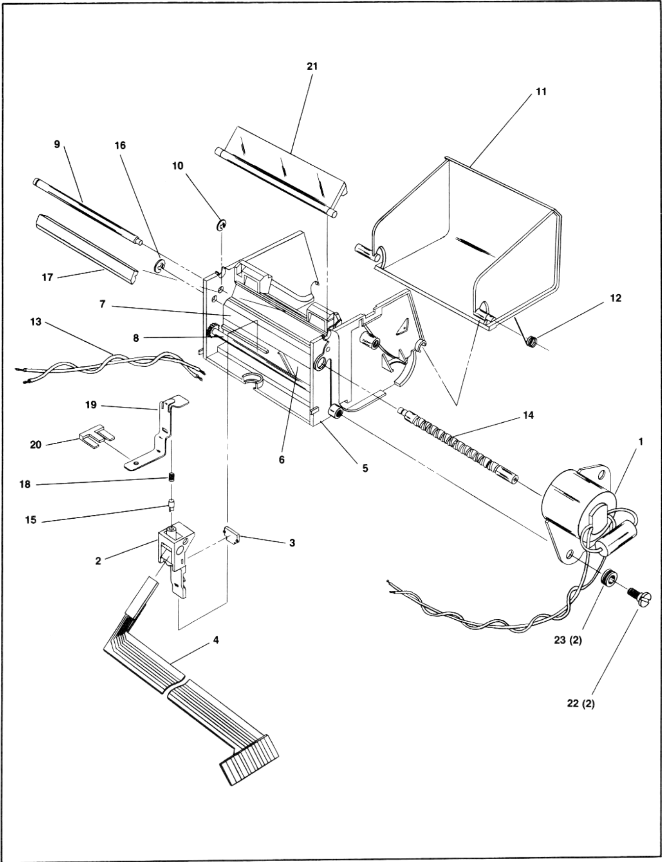
Figure 7-2. Printer Assembly Exploded View
