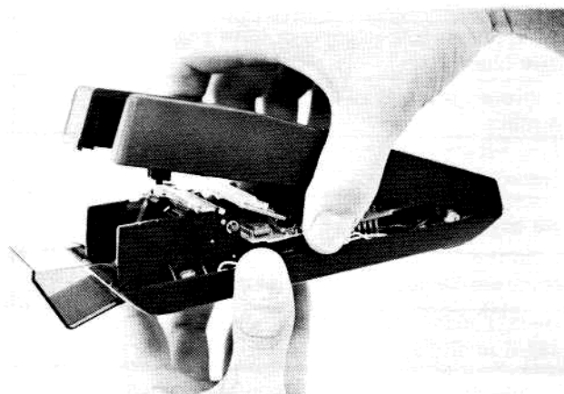
Figure 3-1. Separating Cases
