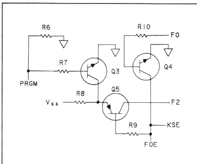
Figure 2-14. Switch Decoding Circuitry
