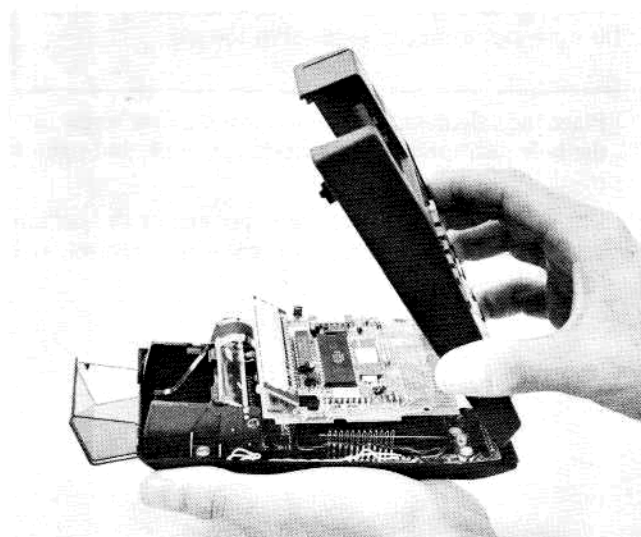
Figure 3-5. Positioning Keyboard/Topcase Assembly Over Bottom Case
