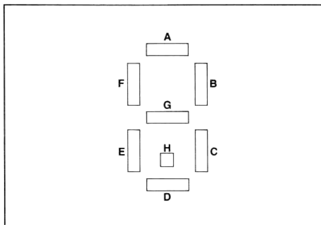
Figure 2-4. Displayed Digit Structure
