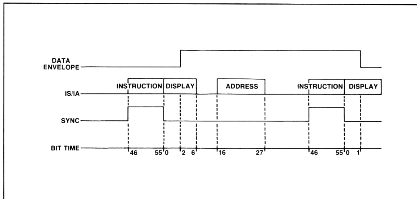
Figure 2-15. DATA, SYNC, and IS/IA Timing
