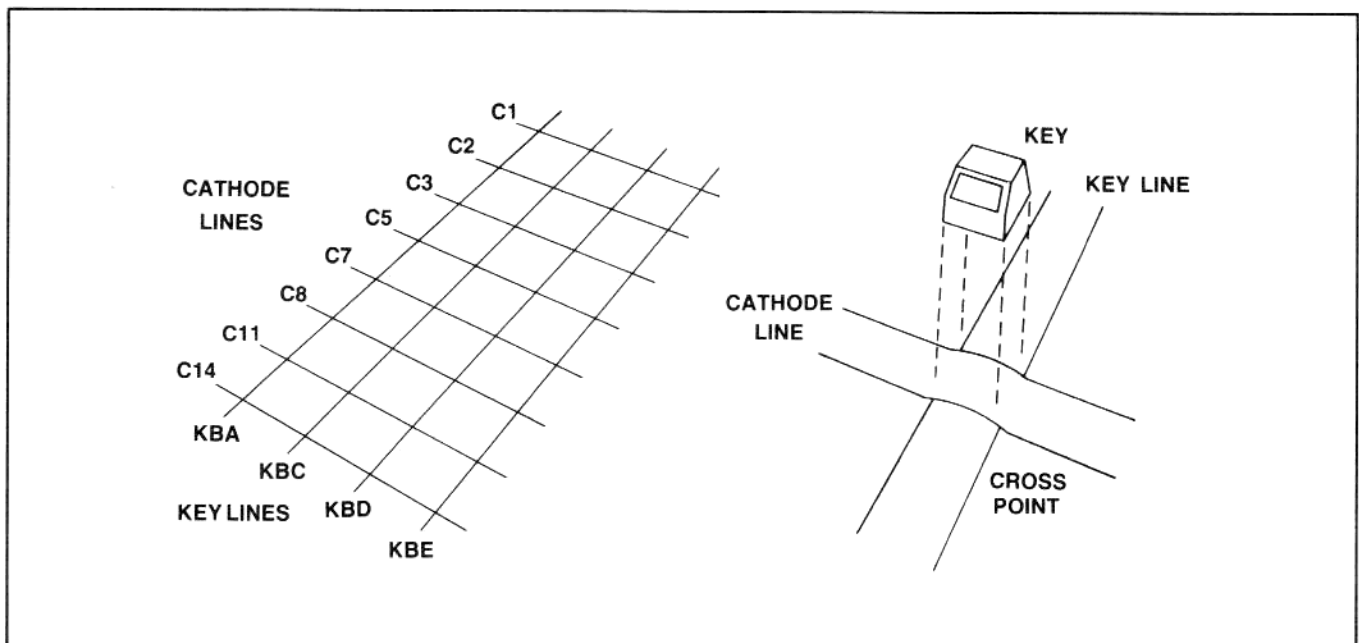
Figure 2-3. Keyboard Operation
