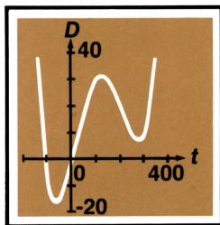
Graph of f(t)
