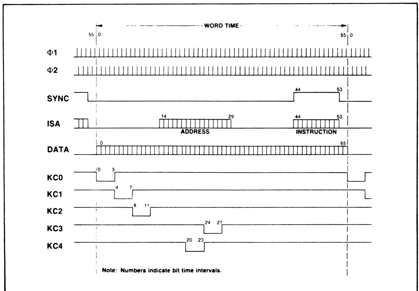
Figure 2-3. System Timing
