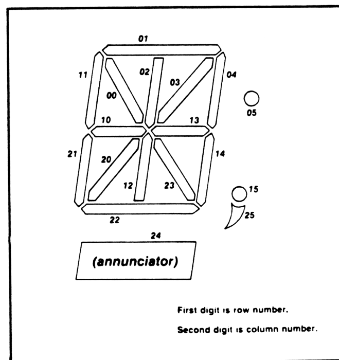
Figure 2-2. Display Character Structure
