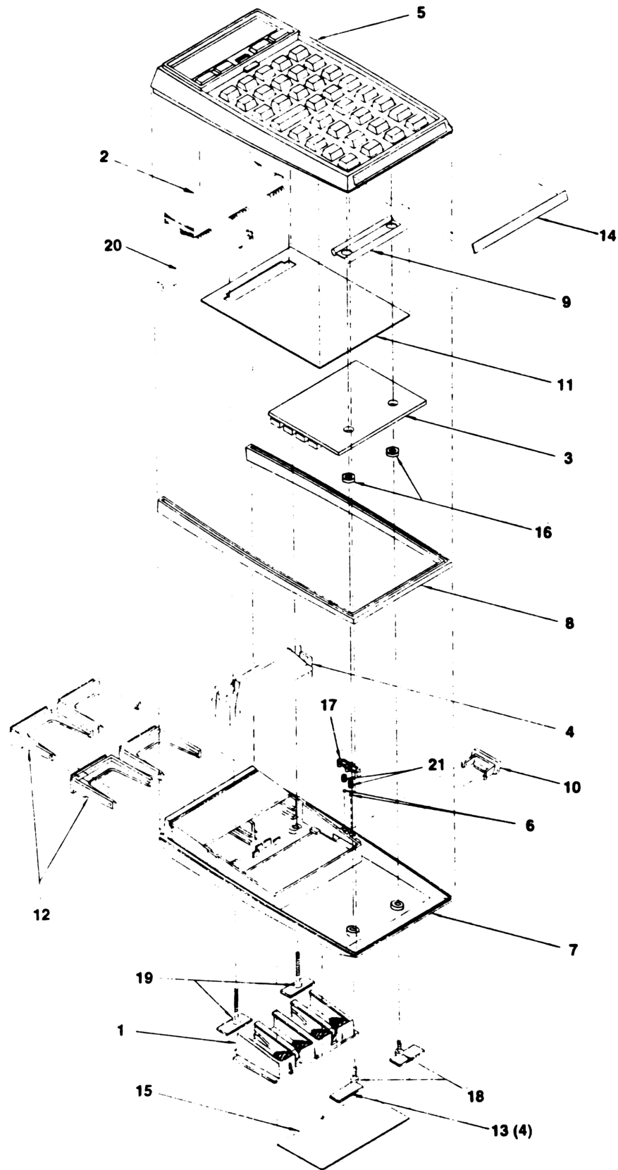
Figure 6-1. HP-41C Exploded View
