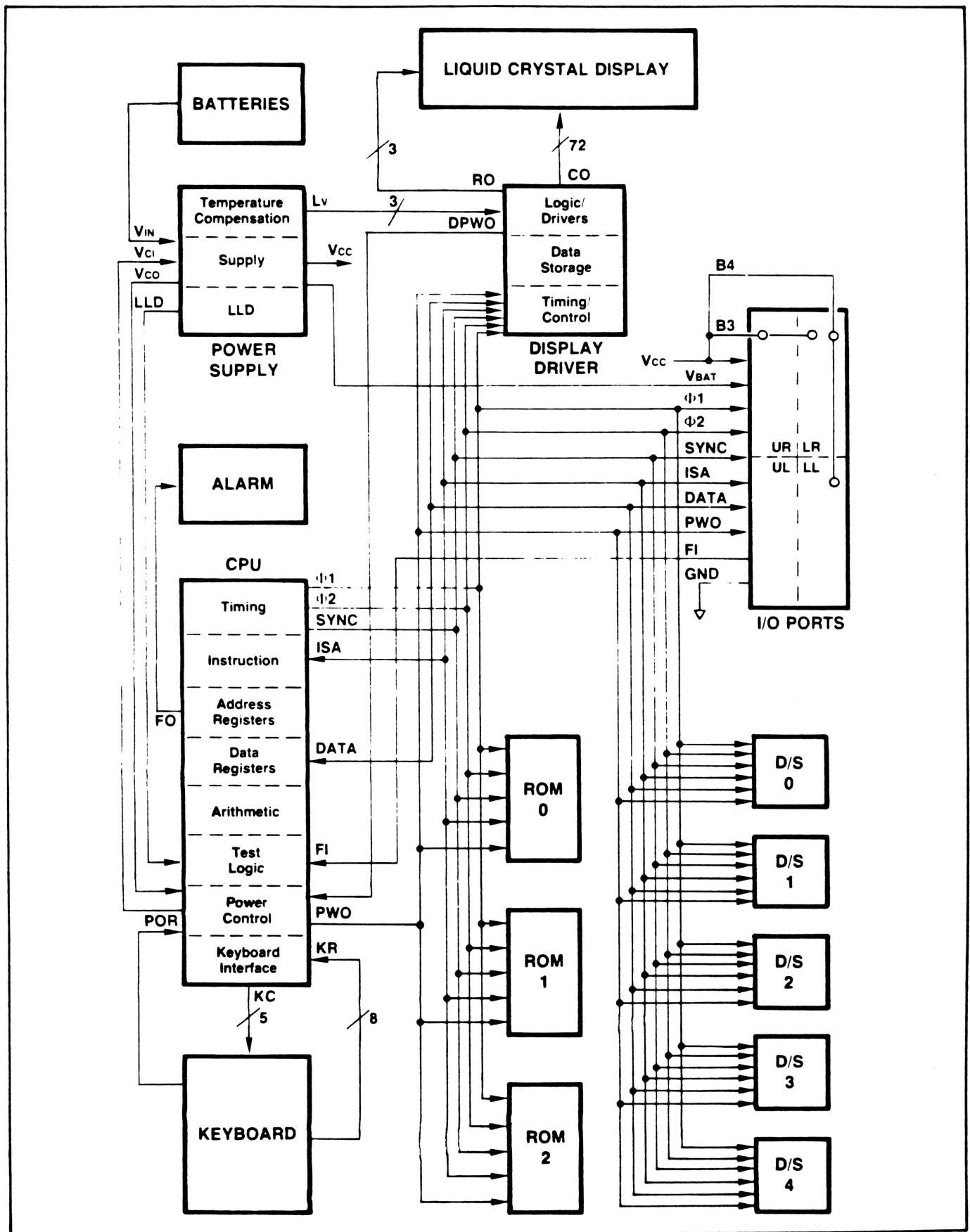
Figure 2-1. HP-41C Block Diagram
